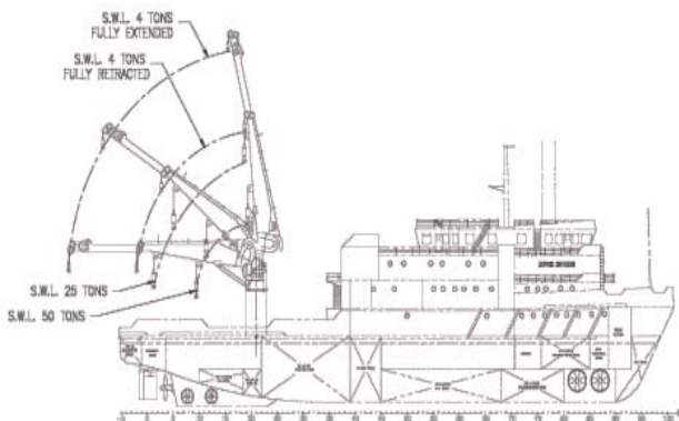
Outboard Profile
