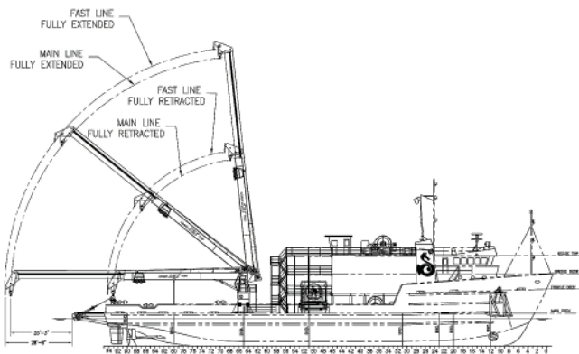
Outboard Profile
