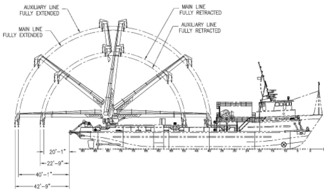
Outboard Profile
