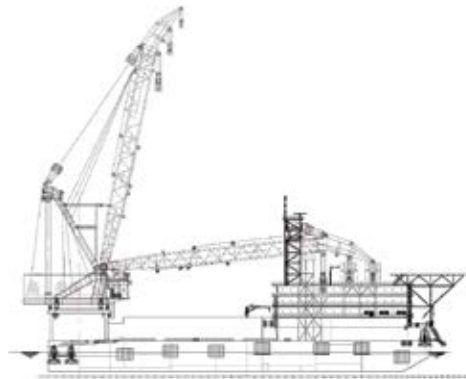
Derrick Barge Elevation
